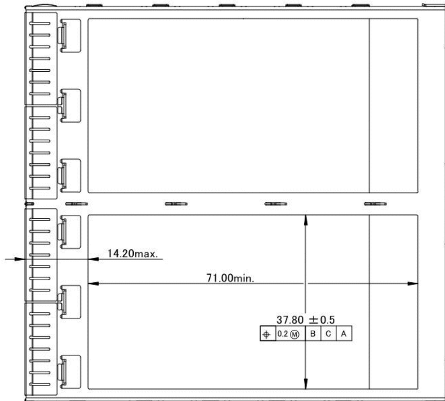
Figure 5-9: Host Cage Top Surface Opening
