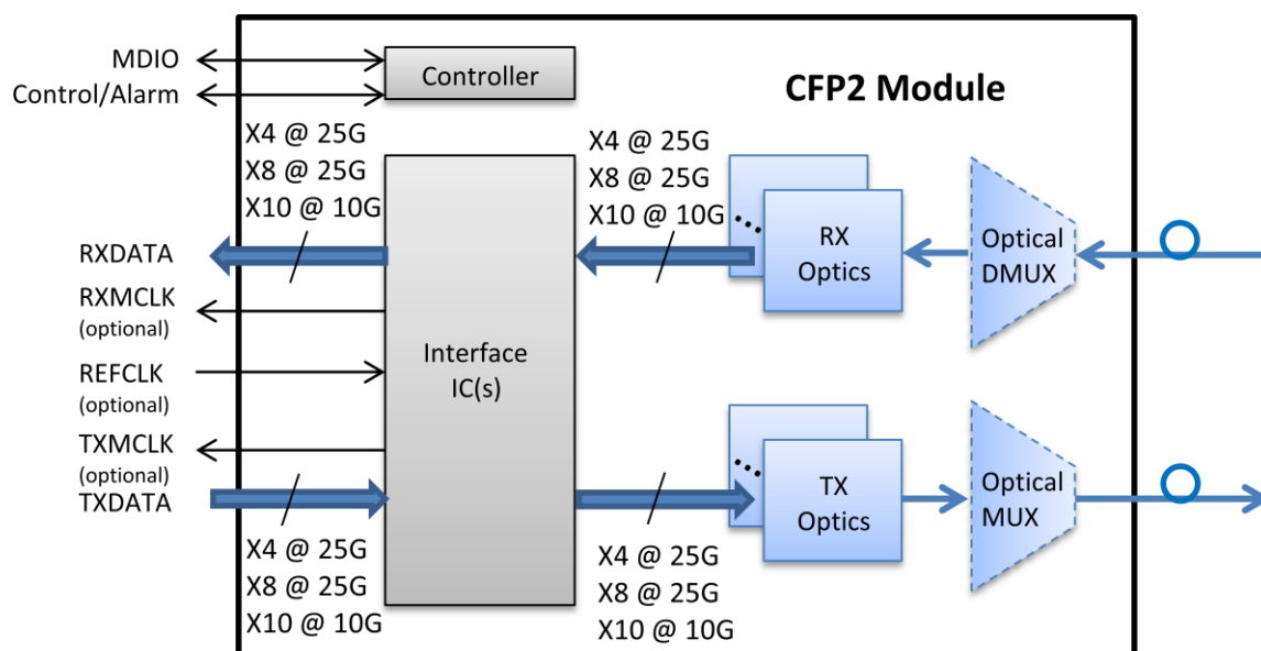
Figure 1-1: CFP2 Functional Block Diagram
