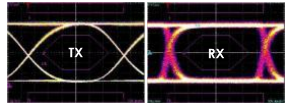
155 Mb/s, 2 23 -1 NRZ Data Eye Pattern
